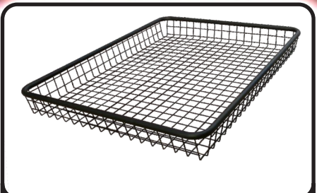
K LBS - K LBM - K LBL L = 1240mm - L = 1310mm - L = 1610mm W = 945mm - W = 1070mm - W = 1220mm H = 130mm - H = 140mm - H = 160mm
